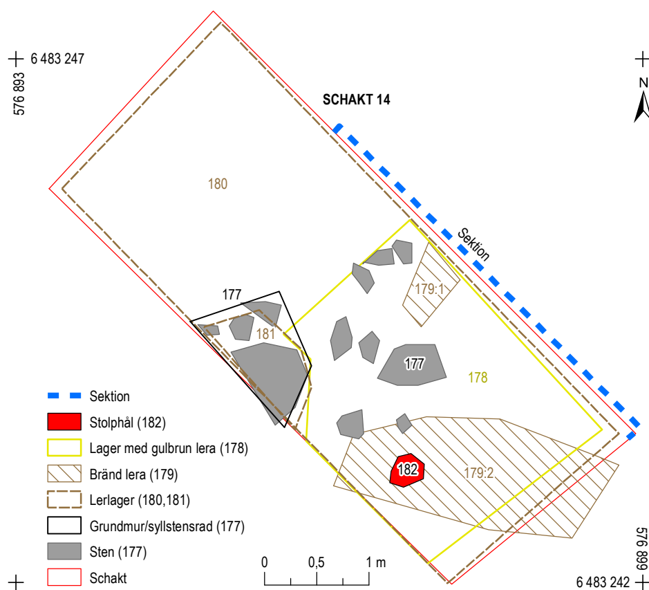
Figur 43. Schakt 14, skala 1:50.
